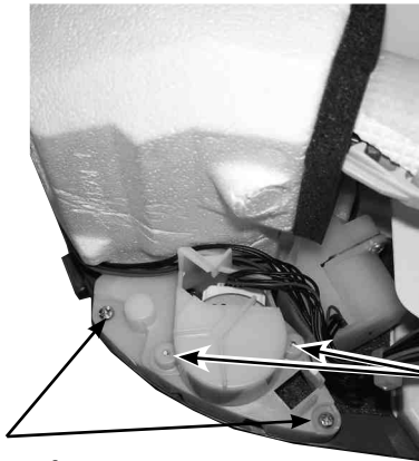
Screws of the horizontal vane motor unit Screws of the horizontal vane motor unit cover
