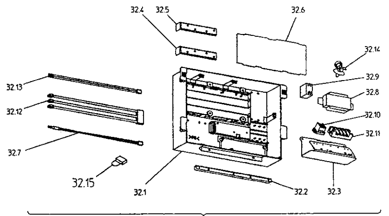
32 SWITCH BOX ASSY
