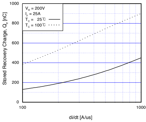
Fig 20. Stored Charge
