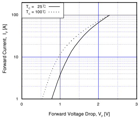
Fig 18. Forward Characteristics
