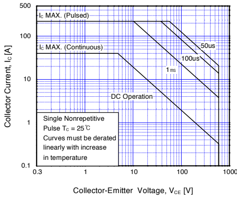
Fig 15. SOA Characteristics
