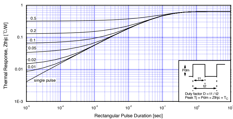
Fig 17. Transient Thermal Impedance of IGBT
